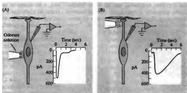
Fig. 17.13. Responses of Isolated Olfactory Cells from the salamander. A patch clamp electrode is used to record whole-cell current. A solution containing 0,1 mV odorant mixture in 100 mM KCl is applied to the cell by a brief (35 ms) pressure pulse. (A) When solution is applied to the cell body, there is a rapid transient inward current due to the increased KCl concentration, followed by a smaller, slower current as the odorant reaches the apical end of the dendrite. The time course of the fast inward current is indicative of the time course of application and dissipation of the electrode solution. (B) When the solution is applied to the dendrite, there is only a small rapid current due to the KCl but a large current due to the odorant lasts for several seconds after the electrode solution has washed away. (After Firestein, Shepherd, and Werblin, 1990.)
