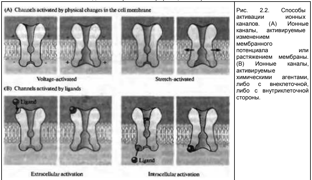
Fig. 2.2. Modes of Channel Activation. The probability of channel opening is influenced by a variety of stimuli. (A) Some channels respond to changes in the physical state of the membrane, specifically changes in membrane potential (voltage-activated) and mechanical distortion (stretch-activated). (B) Ligand activated channels respond to chemical agonists, which attach to binding sites on the channel protein. Neurotransmitters, such as glycine and acetylcholine, act on extracellular binding sites. Included among a wide variety of intracellular ligands are calcium ions, subunits of G proteins, and cyclic nucleotides.
